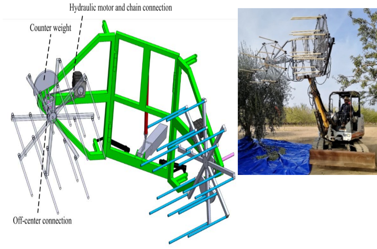
Fig. 7. UC Merced canopy contact harvester head.
