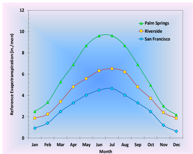
Figure 3- Differences in plant water use in the San Francisco Bay area, Riverside, and Palm Springs due to varying evapotranspiration (ET) rates. Source: Richard Snyder, Department of Land, Air and Water Resources, UC Davis
