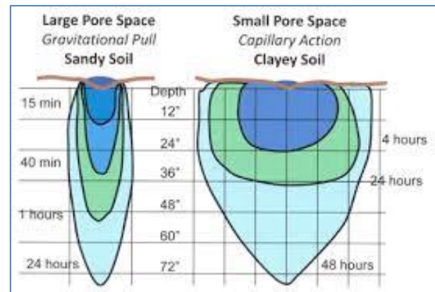
Figure 4 - Comparative movement of water downward and outward in sandy and clay soils
